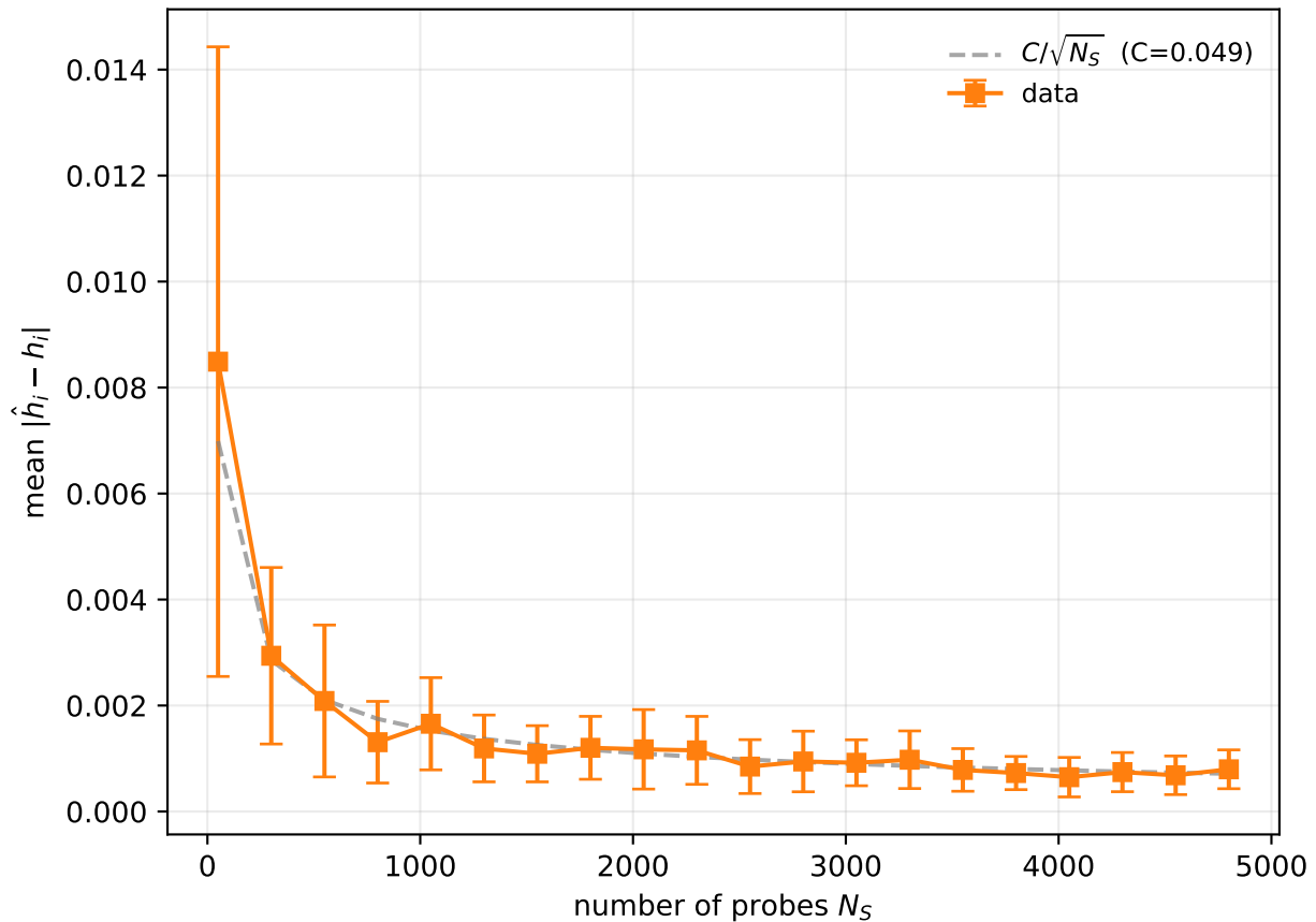
TFIM, n=10 , shots=50000
